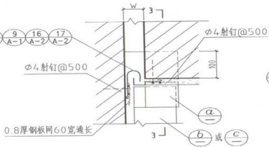
2-2
