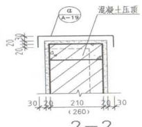
2-2 (压顶无挑出)
